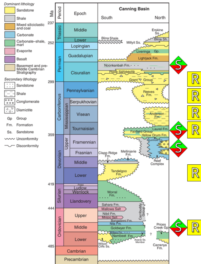
Figure 2: Generalised Paleozoic stratigraphy of the Onshore Canning Basin (after Haines et al. , 2013). “S” means potential source; “R” means potential reservoir, denoting the plays that hypothetically extend offshore that are discussed in the text.
